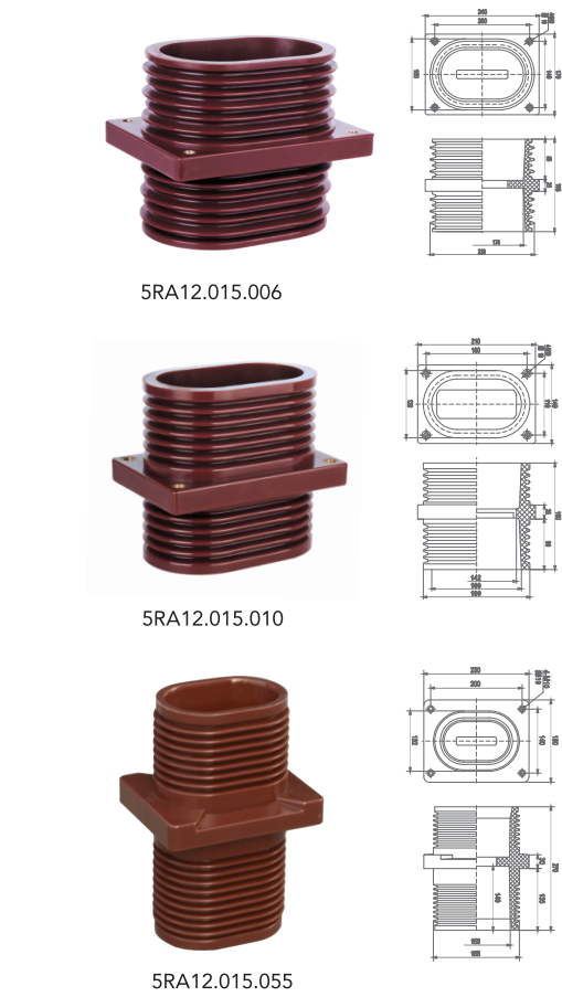
母排参数(BMC/硅橡胶) Busbar Data(BMC/Silicone Rubber)
