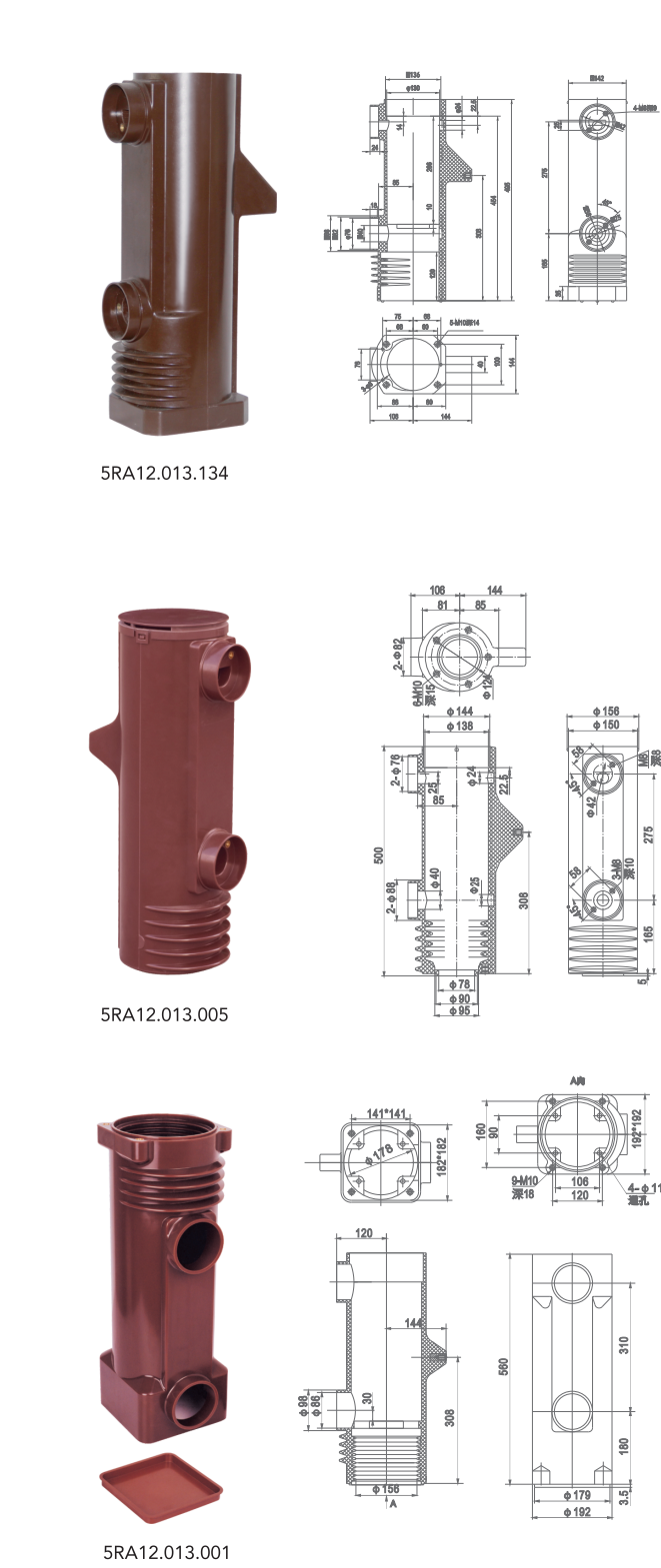
Vs1绝缘筒 Vs1 INSULATING CYLINDER
